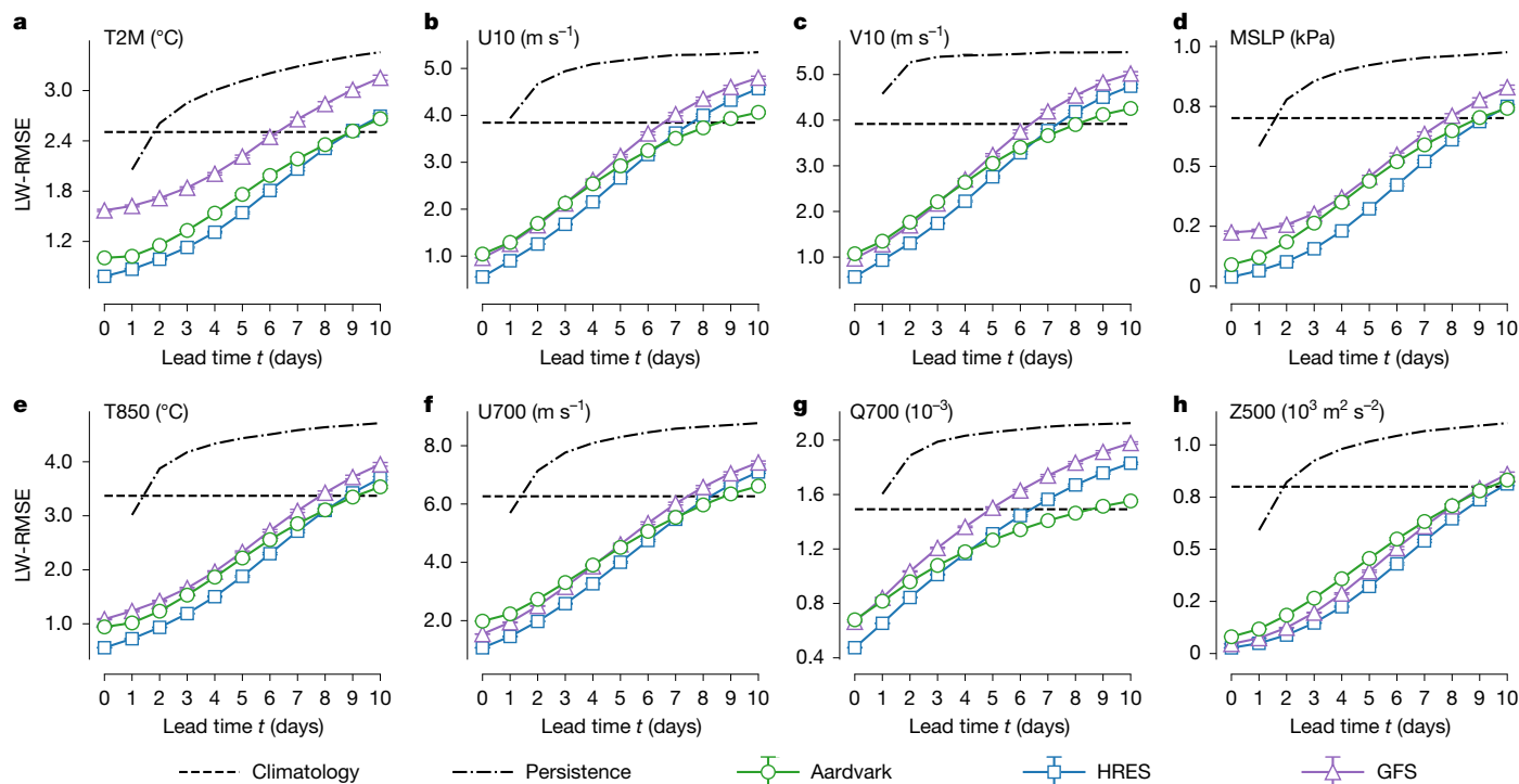
Fig. 2 | Gridded global forecast performance for selected variables.
