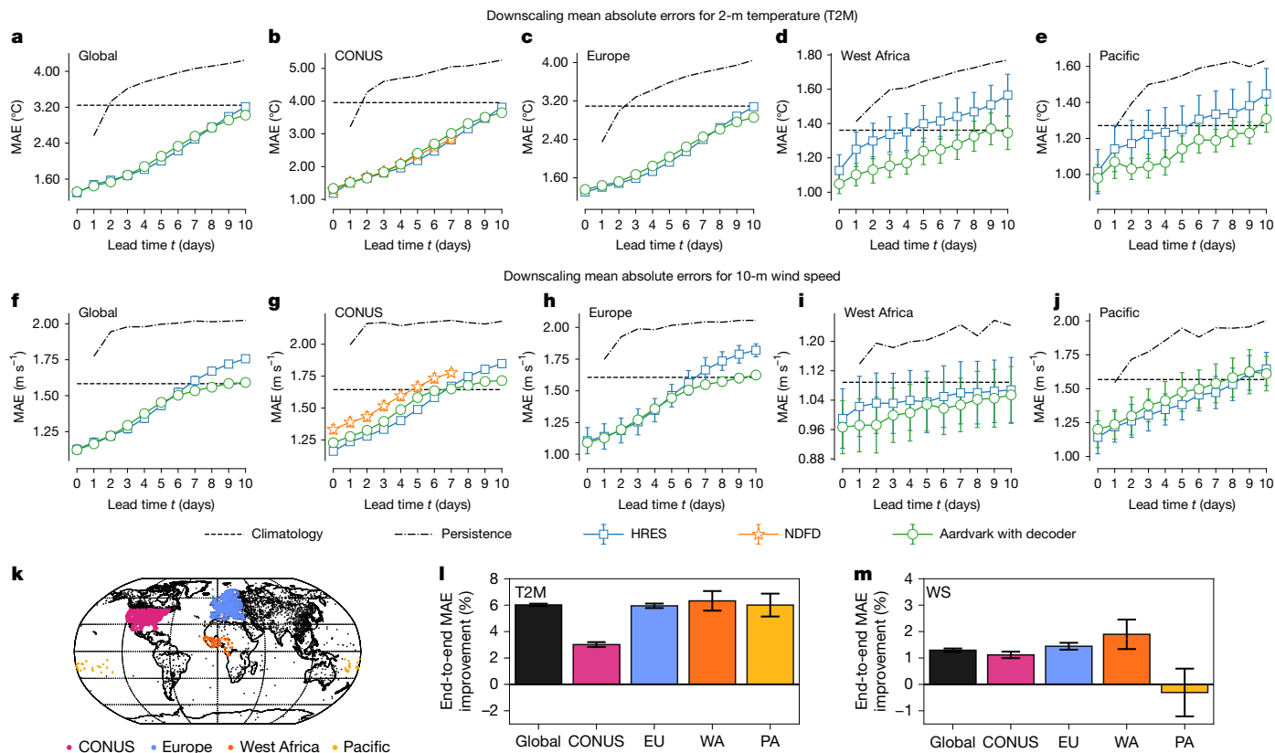
Fig. 5 | Station forecast performance and end-to-end fine-tuning improvements. a–j , The results of station forecasting for the held-out test set (2018) of HadISD data 46 , across different geographic regions (Global, CONUS, Europe, West Africa and Pacific) and predicted variables (2-metre temperature and 10-metre wind speed). Aardvark made predictions at spatial locations observed during training on temporally held-out data, but it can also generate predictions at any arbitrary station location. We compared Aardvark’s forecasts with two state-of-the-art NWP baselines: NDFD 36 for CONUS. We also compared it against a version of HRES 33 that we post-processed using a separate scale and bias term for each station. We report the mean performance of each system
