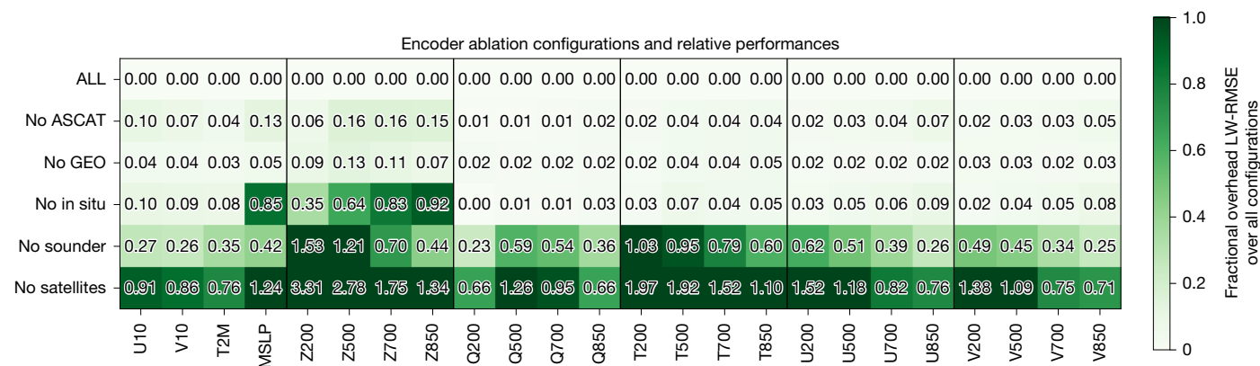
Fig. 4 | Encoder ablation experiments quantifying the impact of each data modality. The results of ablation experiments comparing the latitude-weighted RMSE (LW-RMSE) of the encoder trained with all data sources, both remote sensing 40–45 and in situ sources 46–48 (ALL) to other encoder configurations, including removing the scatterometer data
