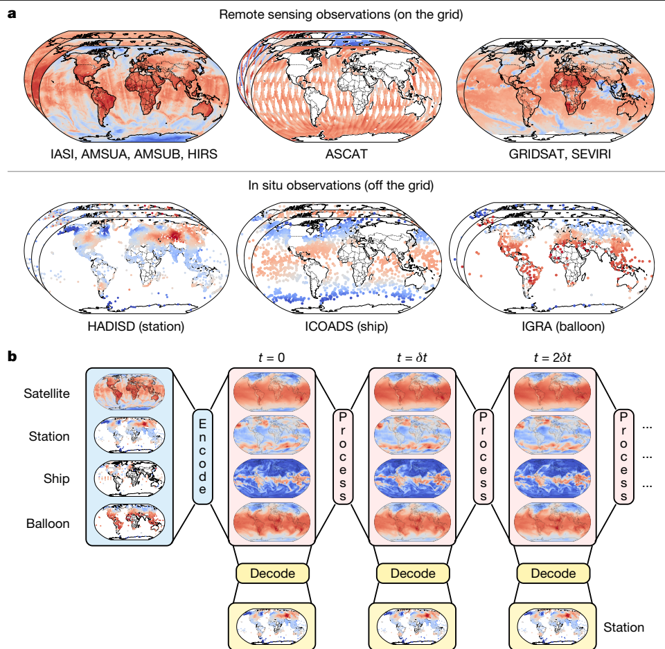
Fig. 1 | Data and operation of Aardvark Weather. a , Different data sources leveraged in Aardvark. The input data consist of observations from remote sensing instruments (top row), which we pre-grid before passing to the model, as well as in situ observations from land and marine observation platforms and radiosondes (bottom row). Each of these data modalities contains several observational variables, of which we selected a subset here for the purposes of illustration. Here we show remote sensing data 40–45 , after performing our gridding step, and raw in situ data 46–48 . Note that the colours in all six plots are meant for illustration purposes. The remote sensing data also include a range of metadata about the measurements, omitted here for simplicity. White areas
